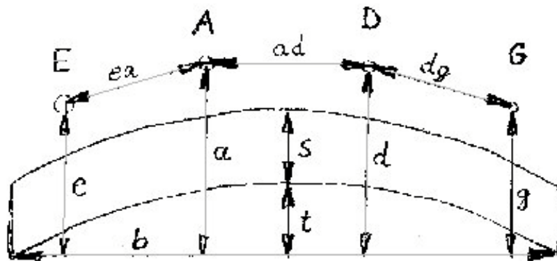
bottom view of the fingerboard
